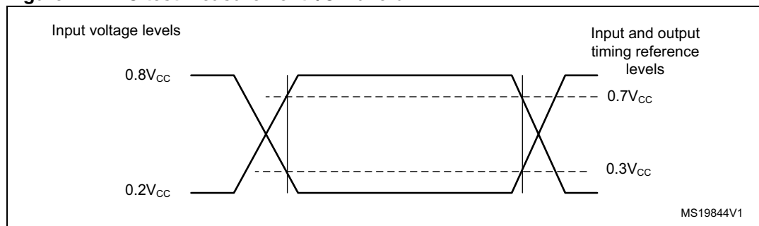
Figure 12. AC test measurement I/O waveform
