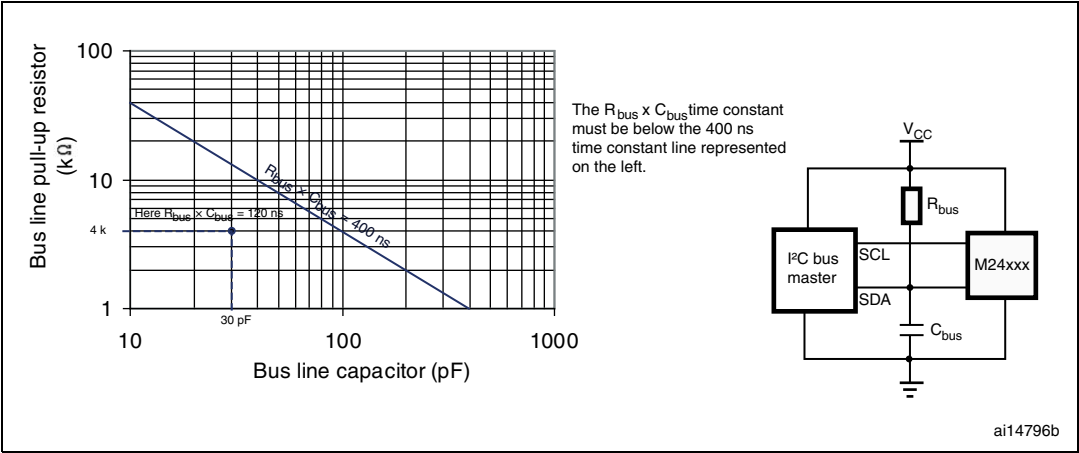
Figure 4. I 2 C Fast mode ( f_C = 400 kHz): maximum R_{bus} value versus bus parasitic capacitance ( C_{bus} )
